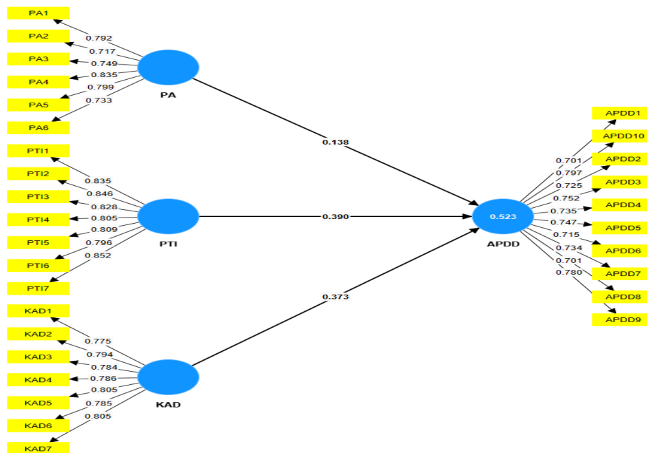
Gambar 1. Uji Outer Loading
