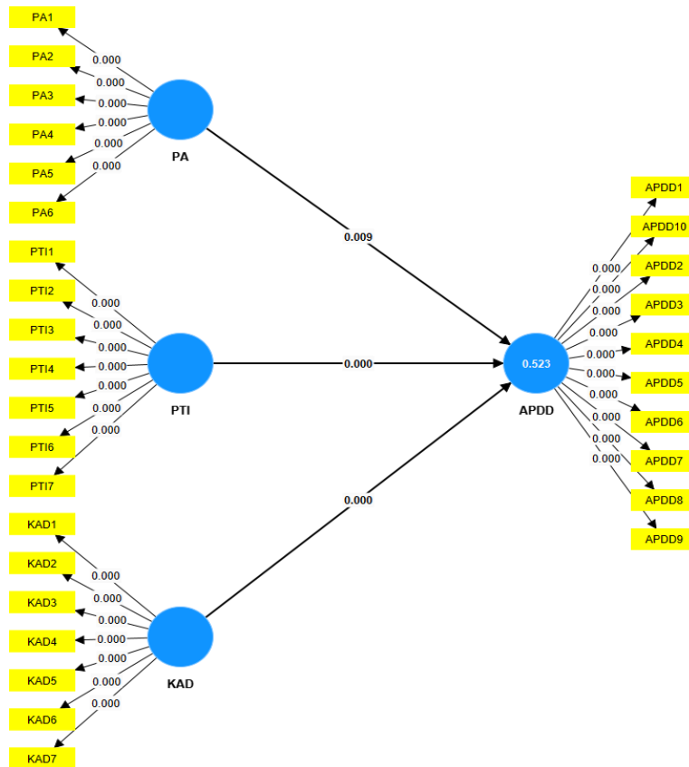
Gambar 2. Structural Inner Model
